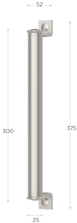
Barrel Pull Handle - KS2000
