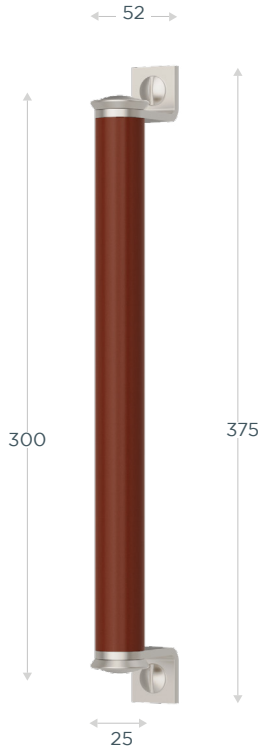
Barrel Stich In Pull Handle - KL2144
