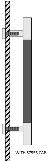
S7555 decorative cap option for covering M10 fastener head
