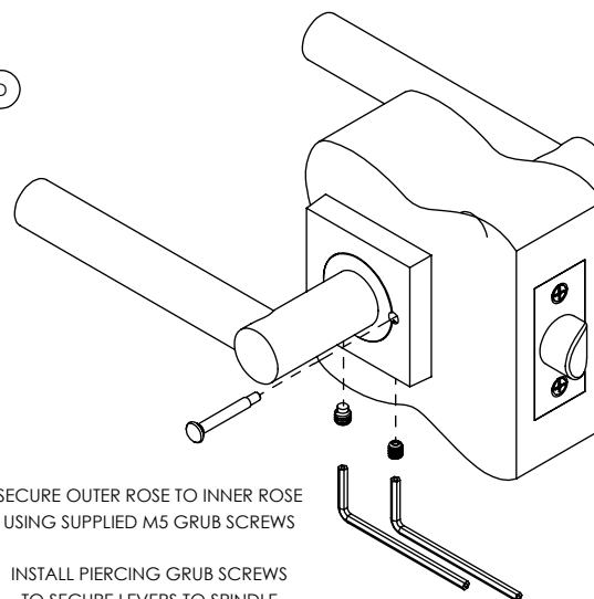
DETAIL A ORIENTATE SPINDLE PIERCING HOLE TOWARDS BOTTOM
