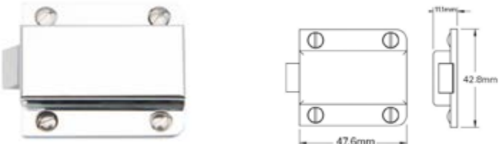
Lux Rim Slam Latch PLK0215
