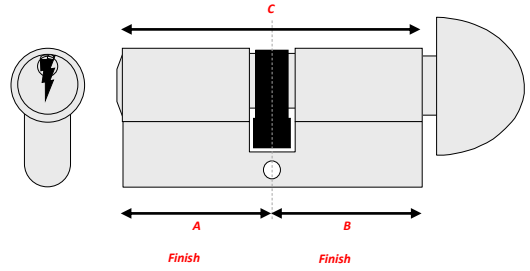
DOUBLE CYLINDER – KEY / TURN Symmetrical
