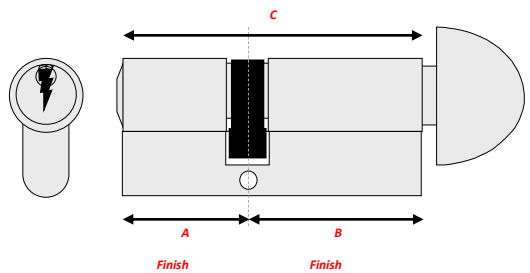
DOUBLE CYLINDER – KEY / TURN Asymmetrical
