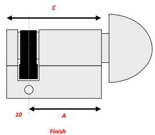
SINGLE CYLINDER – TURN ONLY
