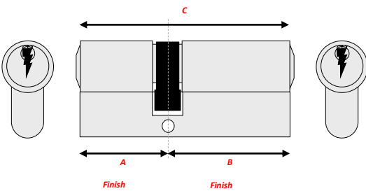
DOUBLE CYLINDER – KEY / KEY Asymmetrical
