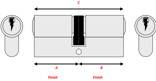
DOUBLE CYLINDER – KEY / KEY Symmetrical
