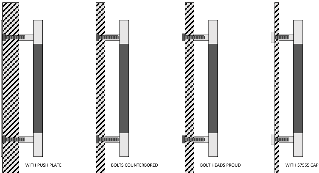
S7555 decorative cap option for covering M10 fastener head
