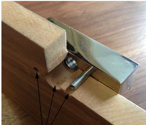
Cross section showing sleeve mounting
